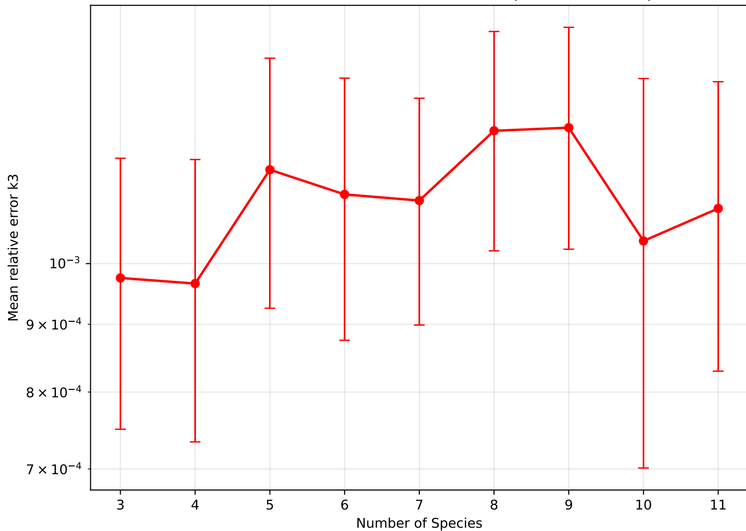
50, 50 — Mean relative error k3 vs number of species (3 to 11 species)
